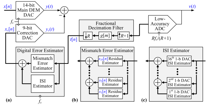
Fig. 2. High-level view of the MNC and ISIC techniques applied to the 14-bit main DEM DAC.
