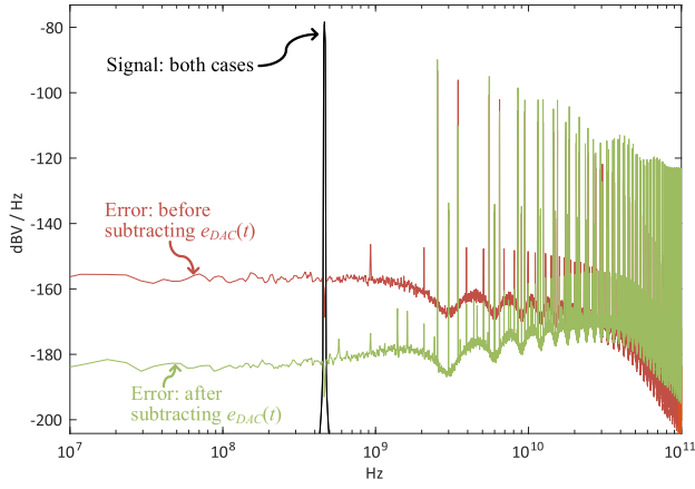
Fig. 7. Output power spectra from a transistor-level simulation of the 14-bit DEM DAC before and after subtraction of e_{DAC}(t) .
