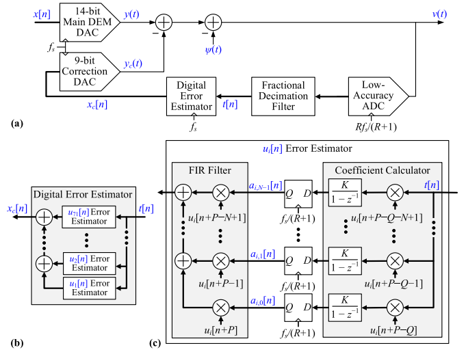
Fig. 9. Modified version of the system of Fig. 2 to facilitate the theoretical analysis presented in Section IV.
