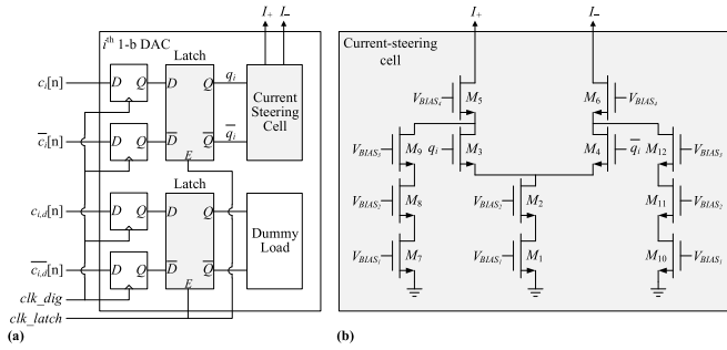
Fig. 8. Circuit details of each 1-bit DAC: a) high-level view, b) current-steering cell details.
