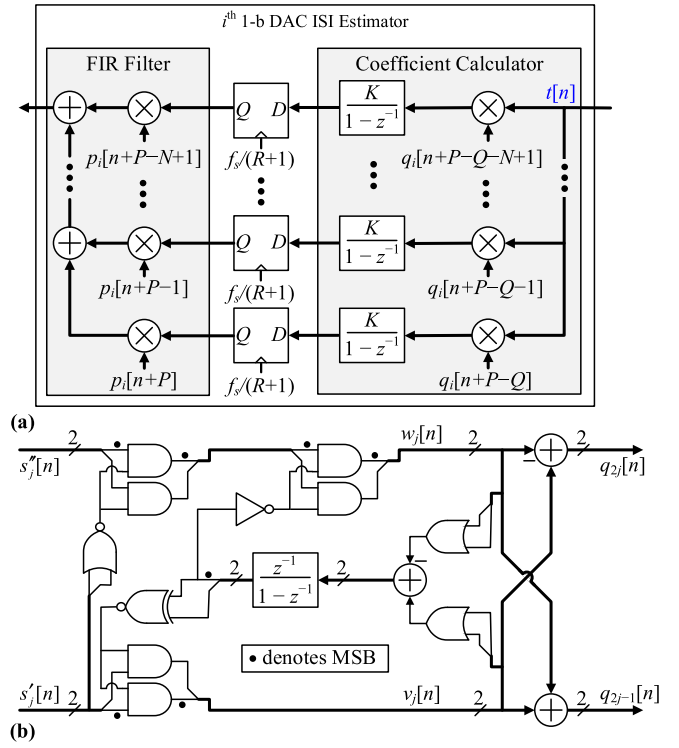
Fig. 4. Details of a) the i th 1-bit DAC ISI estimator and b) the logic that generates the q_i[n] sequences for i = 2j - 1 and i = 2j .
