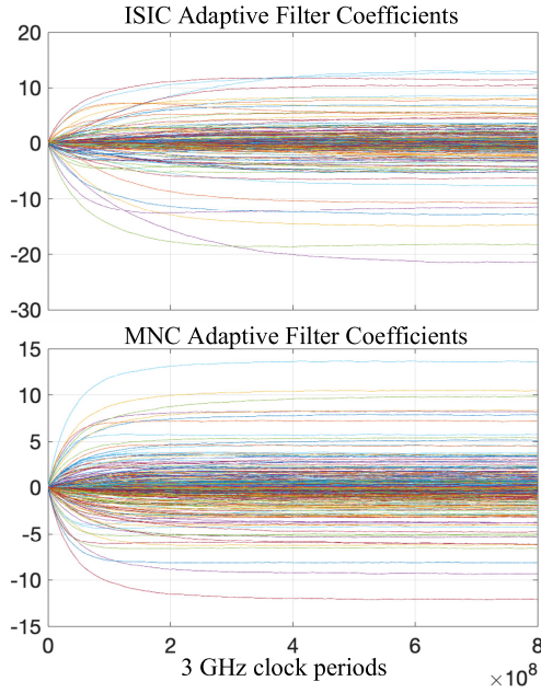
Fig. 6. ISIC and MNC adaptive filter coefficient evolution during foreground calibration.
