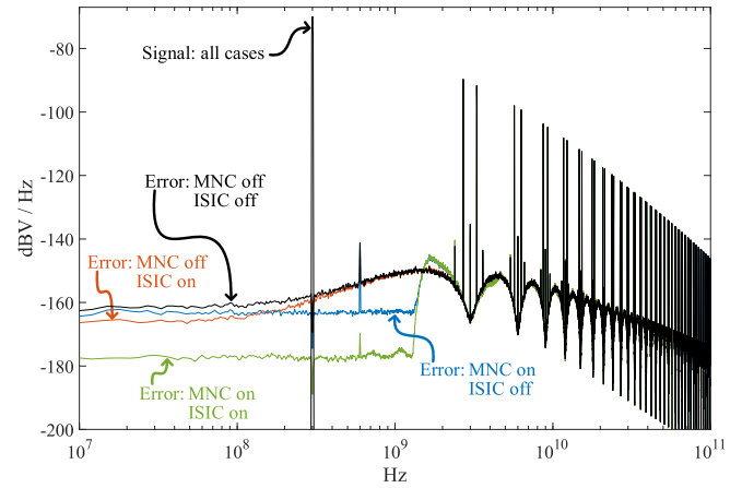
Fig. 5. Output power spectra from behavioral simulations of the system with and without MNC and ISIC enabled.
