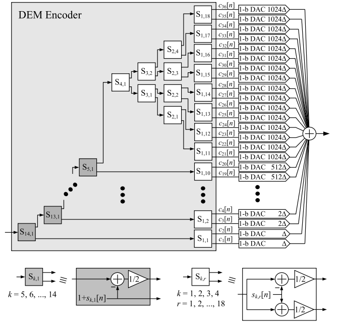
Fig. 1. Details of the 14-bit main DEM DAC.
