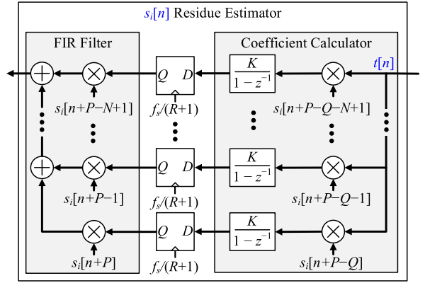
Fig. 3. Details of each s_i[n] residue estimator.
