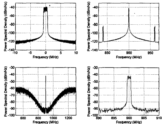
Fig. 2: Computed power spectral densities for upconversion and BPDS encoding of CDMA signal.
